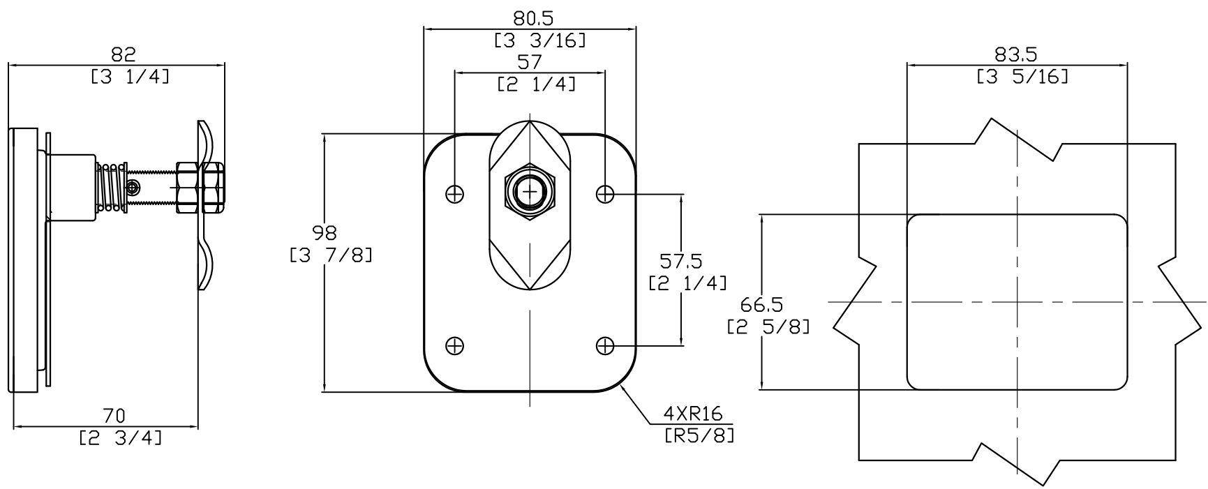
PANEL PREPARATION
